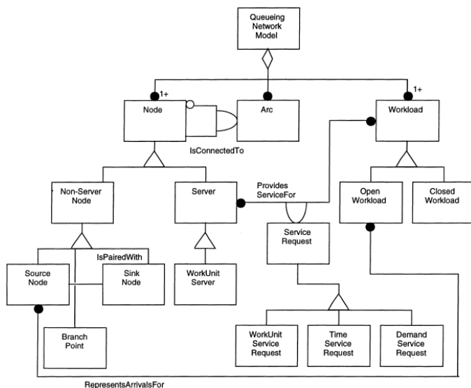
Figure 2: PMIF 1.0 Metamodel
