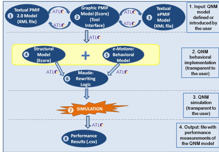
Figure 5: xQNM Architecture
