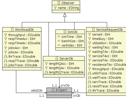
Figure 9: Observers metamodel
